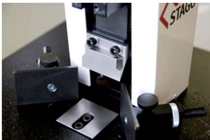
ESM 20 fitted with extra-wide punching knife
