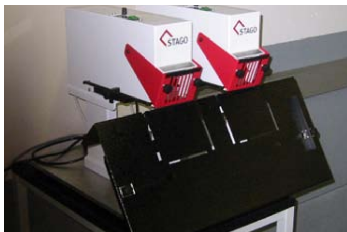
HM 6 fitted with 2 stapling heads in 180mm custom spacing
